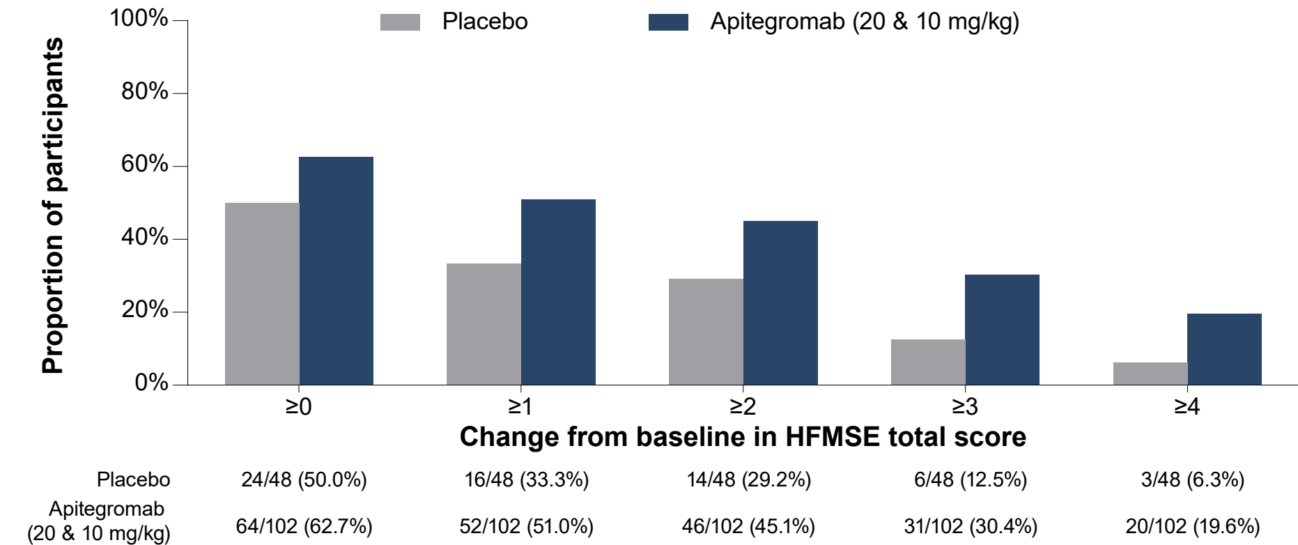
Figure 5. Any point change from baseline in HFMSE total score at month 12 (2-12 population)
